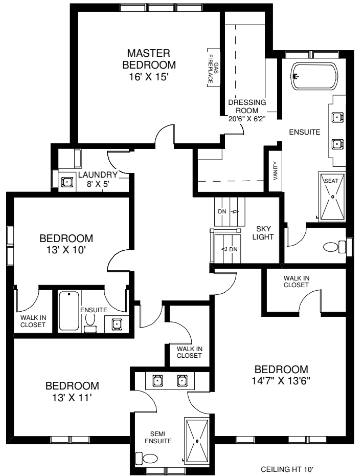
CEILING HT 10' SECOND FLOOR APPROXIMATELY 1,750 SQ FT
