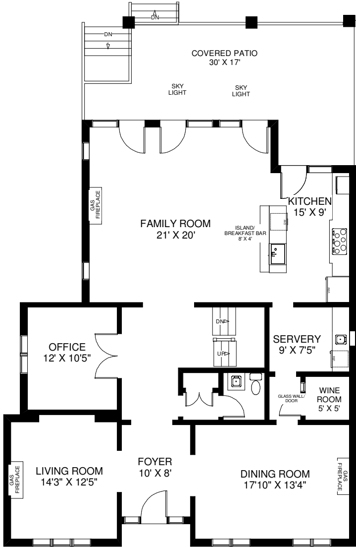
MAIN FLOOR APPROXIMATELY 1,750 SQ FT
