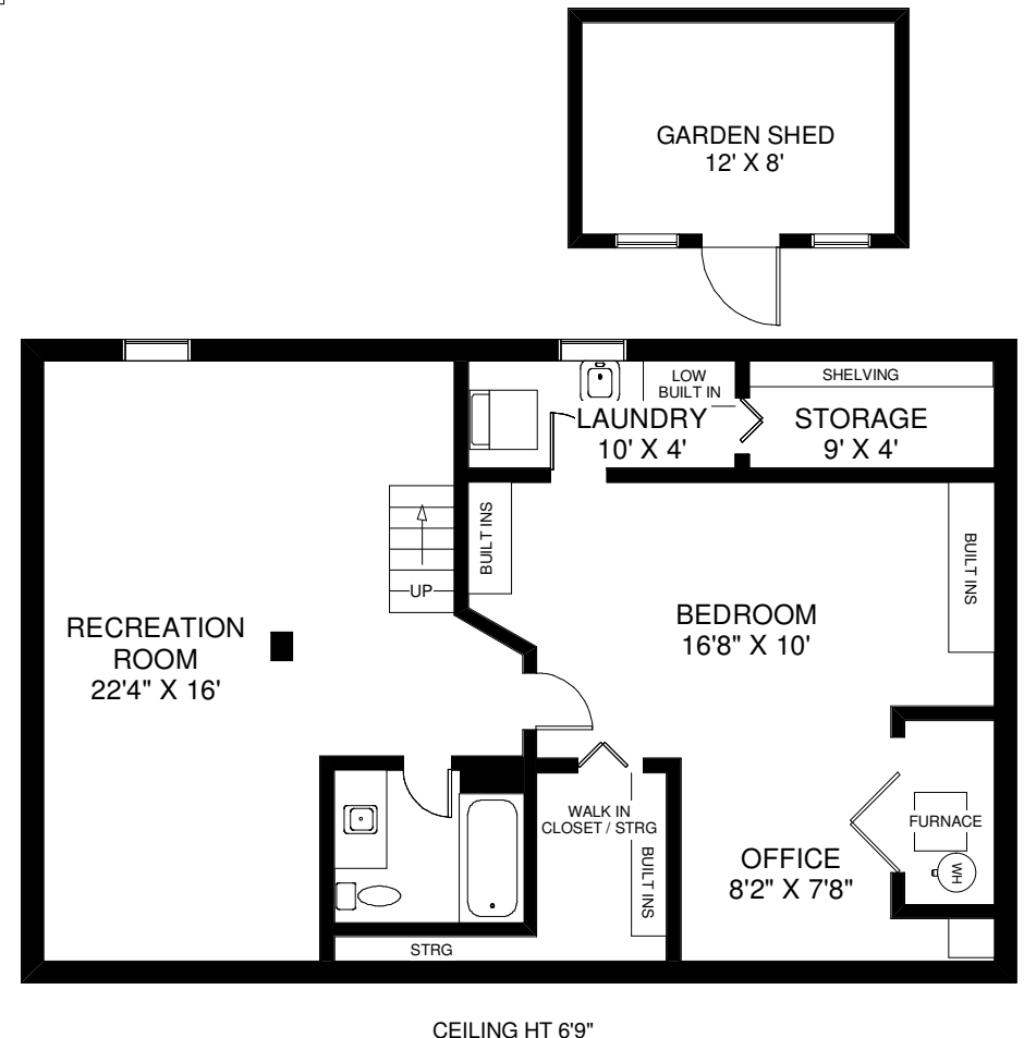
LOWER FLOOR APPROXIMATELY 935 SQ FT
