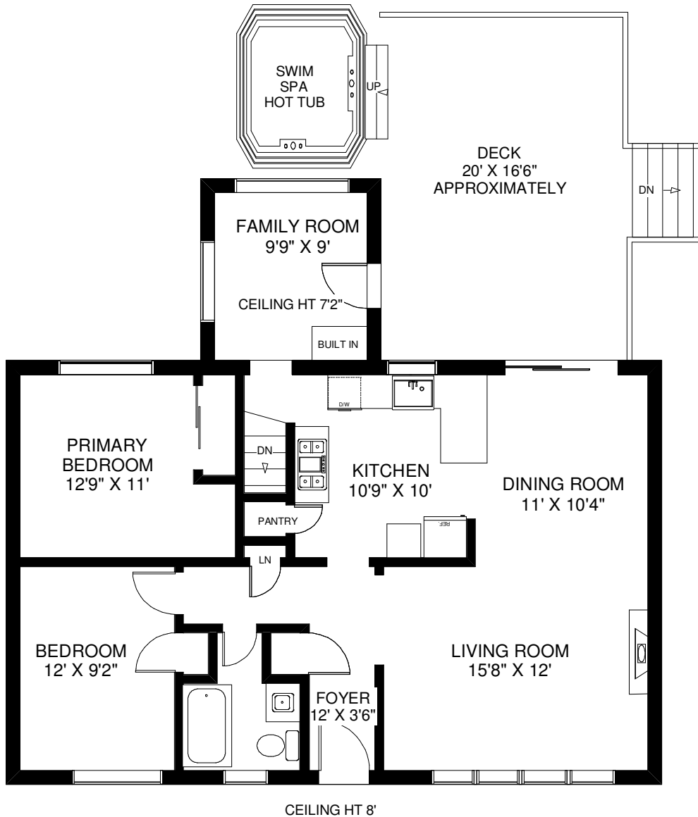
MAIN FLOOR APPROXIMATELY 1,050 SQ FT
