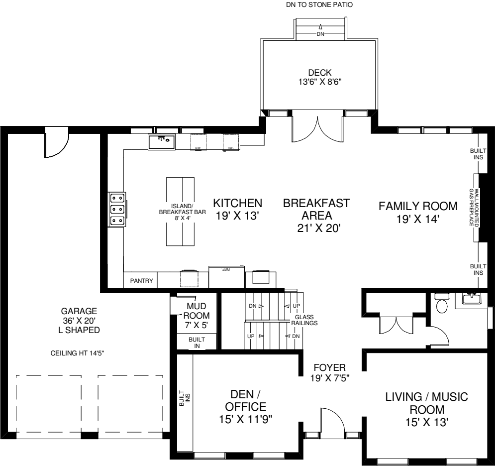
MAIN FLOOR APPROXIMATELY 1,900 SQ FT
