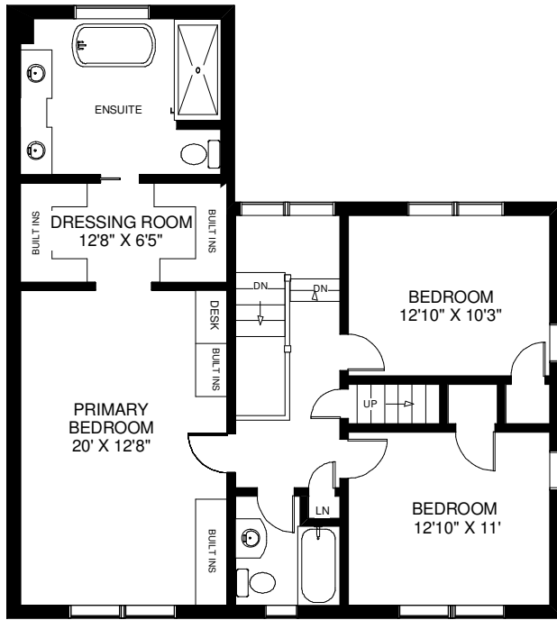
SECOND FLOOR APPROXIMATELY 1,115 SQ FT
